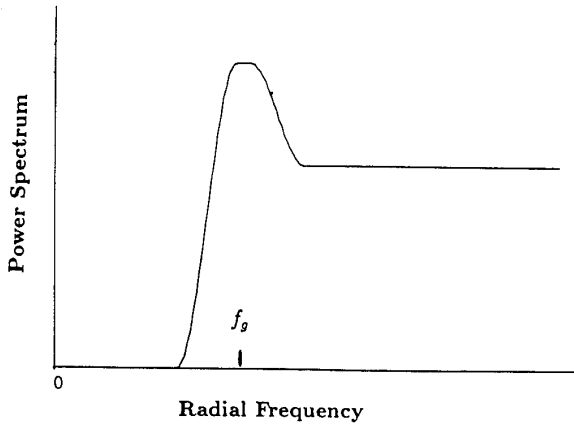
Figure 1. Blue noise power spectrum.
