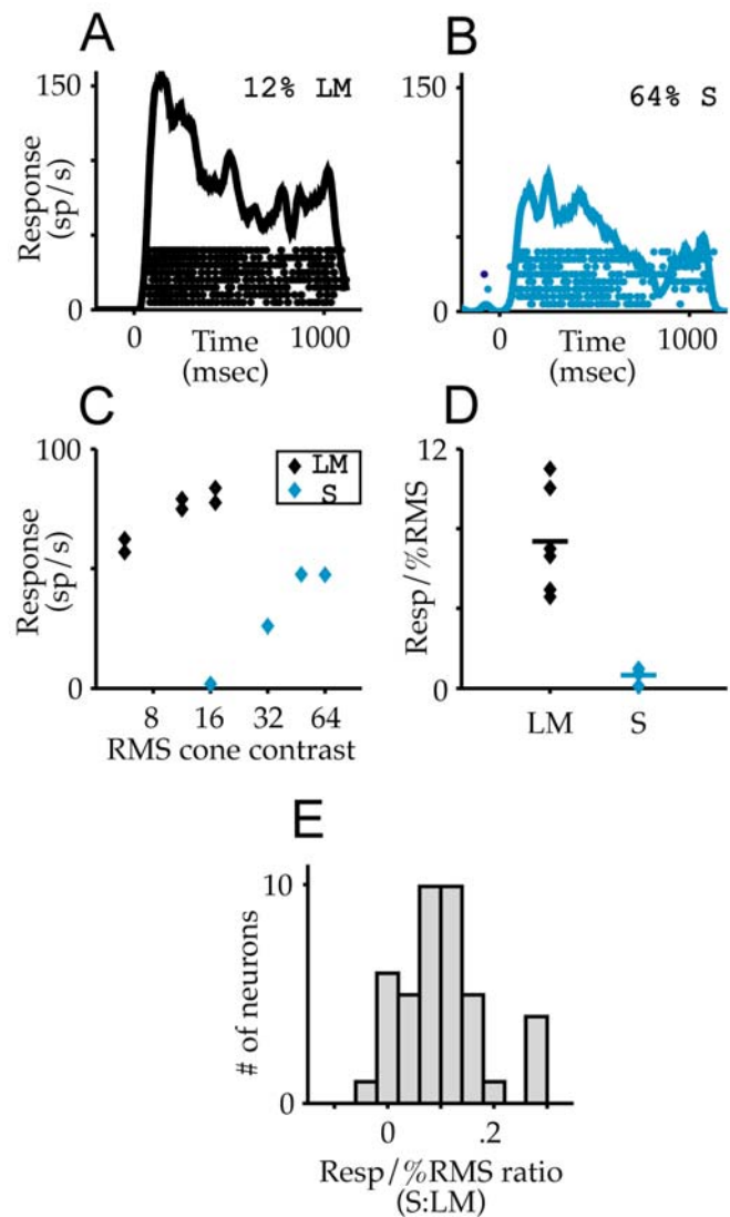
Figure 4. Response magnitude. Relative response magnitude to S- and L,M-cone stimuli. A. Raster and PSTH for one neuron at 12% L,M-cone contrast. B. Raster and PSTH for the same neuron at 64% S-cone contrast. C. Average response (firing rate during stimulus presentation) for the same neuron for several levels of L,M- and S-cone contrast, plotted as a function of RMS cone contrast; each data point represents one stimulus condition. Pairs of points for L,M-cone contrast are for in phase and out-of-phase stimuli. D. Response-per-unit-RMS for each of the trial conditions shown in C. Solid lines mark average response-per-unit-RMS. E. Distribution of the ratio (S : L,M) of average response-per-unit-RMS for the 42 neurons in the primary data set.
