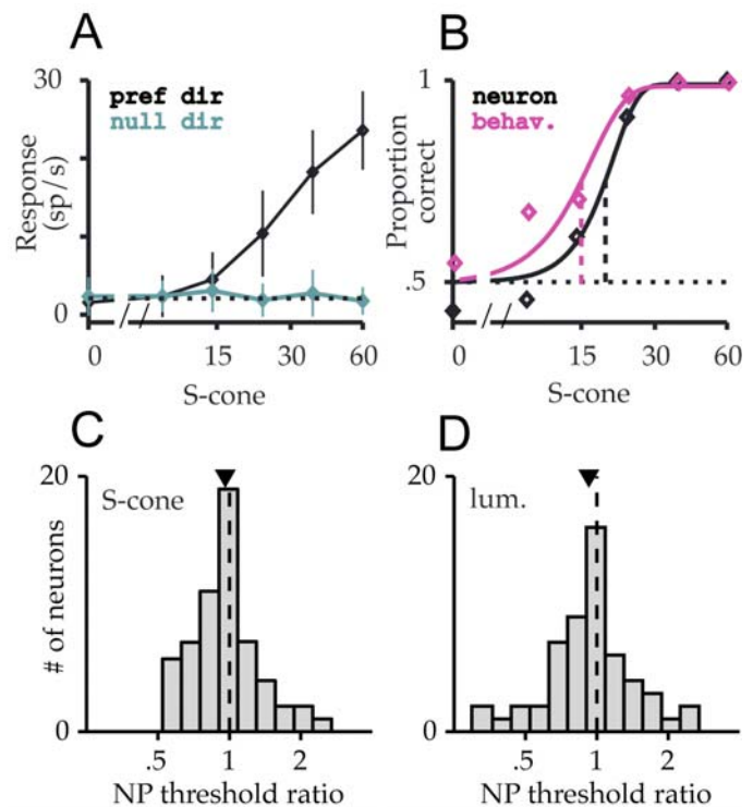
Figure 11. Neurometric-psychometric comparison. A. Average response (firing rate during stimulus presentation) for one neuron as a function of S-cone contrast, for preferred- and null-direction motion. Error bars denote standard deviation. Dashed line indicates spontaneous firing rate. B. Neurometric function (black) derived from the data in A, with the psychometric function (magenta) for the monkey overlaid. Vertical dashed lines indicate contrast threshold. Horizontal dashed line indicates chance performance level. C. Distribution of the neurometric-psychometric (NP) threshold ratio for S-cone contrast stimuli. Black triangle marks average NP ratio across all cells. Vertical dashed line marks a ratio of 1. D. Distribution of the NP threshold ratio for luminance contrast stimuli. Symbol and dashed line as in C.
