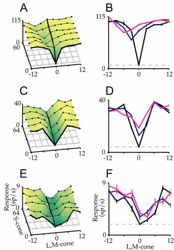
Figure 5. Types of neural response profiles. Three neurons are shown that illustrate the range of response profiles observed. For each cell, two views are displayed: a 3D surface plot, and three 2D slices at different S-cone contrast levels. In the surface plots, heavy lines follow the purely S- and L,M-cone contrast response functions, and data points are indicated by black dots. The flat mesh grid in the 3D plots and the dashed line in the 2D slices plots indicate the spontaneous firing rate. The color scale indicates relative response amplitude, running from zero to the maximum firing rate of each cell. A,B. Summation. C,D. Independence. E,F. Opponency.
