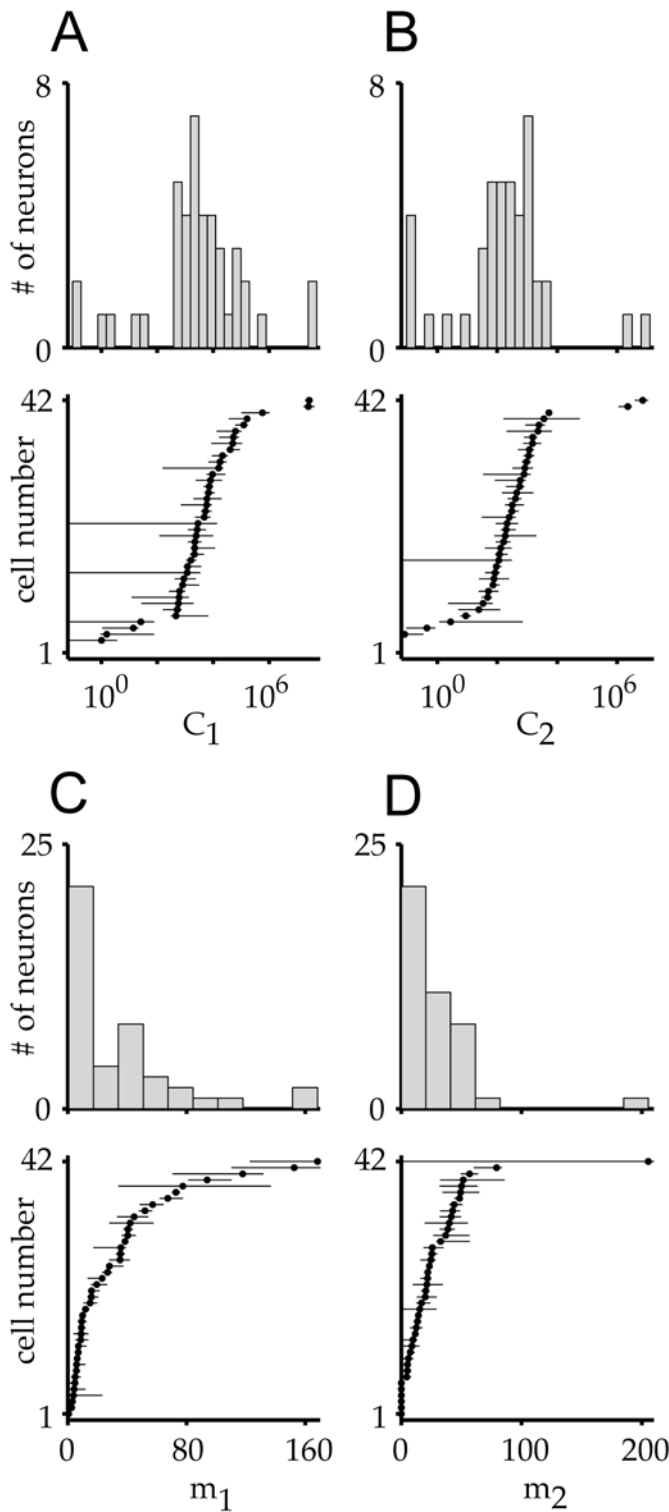
Figure 9. Range and confidence intervals for coefficients of the model fits. A. Distribution (upper panel) and 95% confidence intervals (lower panel) for coefficient C_1 . Mean 2764, median 1.29 \times 10^6 , range <.01 to 2.72 \times 10^7 . B. Coefficient C_2 . Mean 204.9, median 2.25 \times 10^5 , range <.01 to 7.16 \times 10^6 . C. Coefficient m_1 . Mean 17.78, median 34.09, range 0.58 to 168.22. D. Coefficient m_2 . Mean 20.92, median 27.48, range <0.01 to 205.4.
