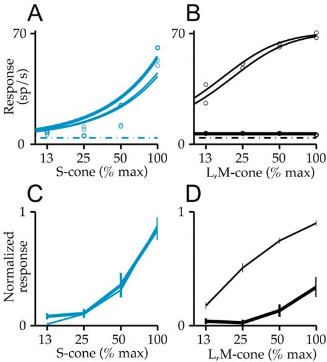
Figure 3. Cone-isolation control experiment. A. S-cone contrast response functions, plotted against percent maximum contrast, for one neuron, obtained before, during and after adaptation to the yellow light. Heavy line: yellow light condition. Spontaneous firing rate is indicated by the horizontal dotted line. B. L,M-cone contrast response functions for the same neuron, plotted as in A. C. Population average ( n=17 ) of the normalized S-cone contrast response function, plotted against percent maximum contrast. Heavy line indicates the yellow light condition; the regular line indicates the average response during the pre- and post-adaptation conditions. Error bars are standard error of the mean. D. Population average of the normalized L,M-cone contrast response function, plotted as in C. Maximum contrast varied from cell to cell so as to capture the dynamic range of the neuron's response, varying primarily as a function of receptive field eccentricity. Maximum L,M-cone contrast varied from 5-30%; maximum S-cone contrast varied from 40-80%. For each neuron, S- and L,M-cone contrast trials were randomly interleaved within a block.
