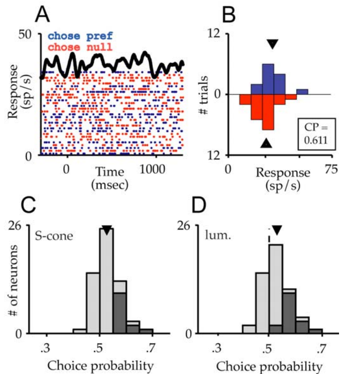
Figure 12. Choice probability. A. Raster and PSTH for one neuron, for 4% S-cone contrast stimuli moving in the preferred direction. Rows of the raster are color-coded according to whether the monkey chose the preferred (blue) or null (red) direction at the end of the trial. B. Distributions of average firing rate for the trials shown in A, for chose-preferred and chose-null subsets. Black triangles mark the mean of each distribution (blue, 30.60 sp/s; red, 26.33 sp/s). C. Distribution of the CP value, computed across all trials, for each neuron in the data set, for S-cone contrast stimuli. Black triangle marks the mean of the distribution. Darker shading indicates neurons that were individually significant (greater than 0.5). D. Distribution for luminance contrast stimuli. Symbol and shading as in C.
