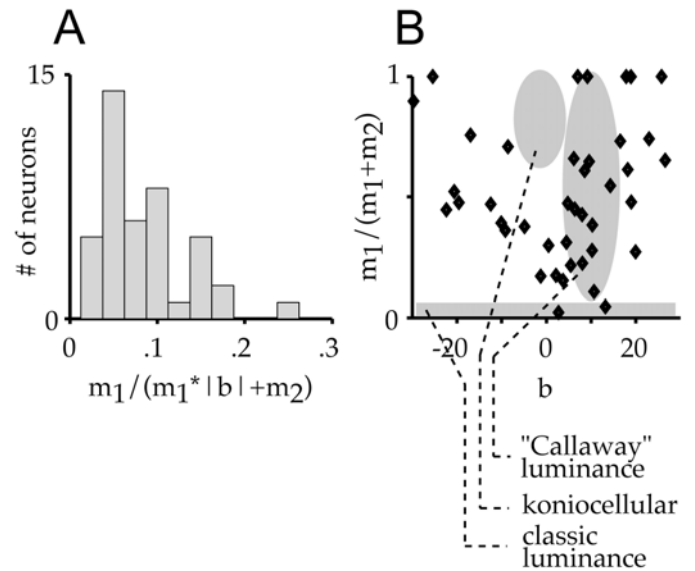
Figure 10. Further analysis of parameters of the model fits. A. Distribution of the weight of S-cone contrast relative to total L,M-cone contrast in the model fits, captured by the value of m_1/(m_1 * |b| + m_2) . B. Scatterplot of the relative weight of the first and second term of the model, captured by the value of m_1/(m_1 + m_2) , plotted as a function of coefficient b . Gray ovals indicate regions of this space where neurons in different color pathways would fall (see Results).
