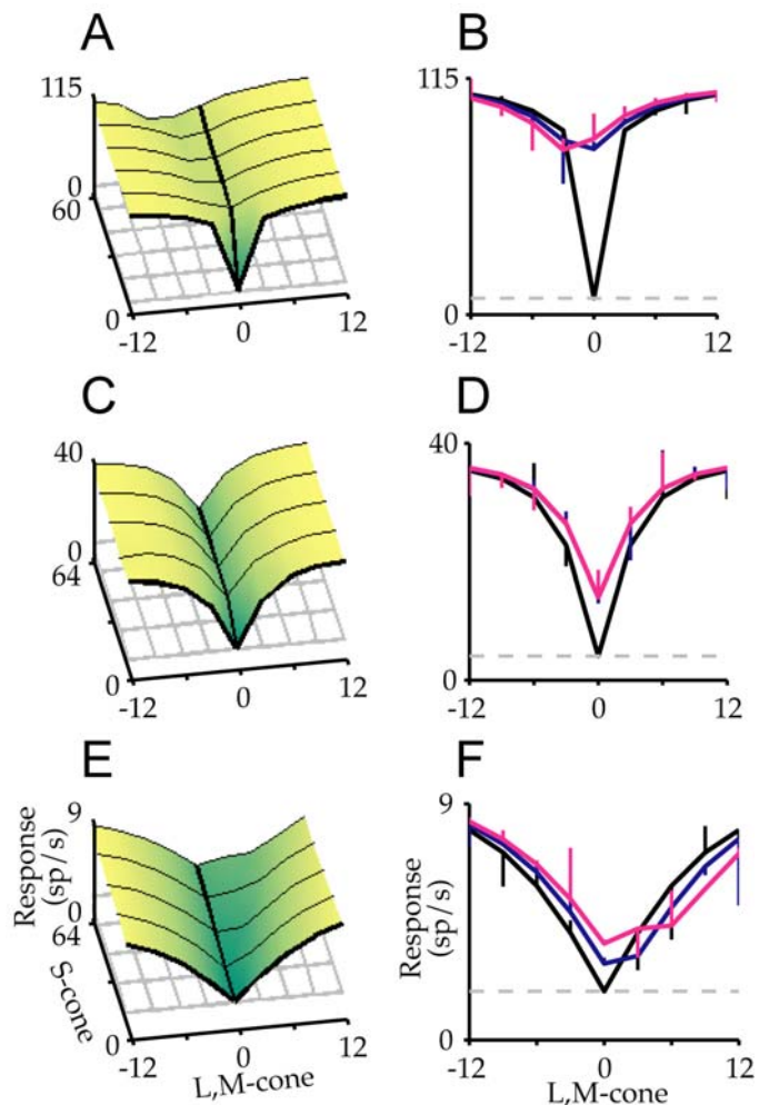
Figure 6. Cone model fits. Cone model fits for each of the neurons shown in Figure 5. Each panel corresponds to the same panel in Figure 5. Vertical bars in 2D slices plots indicate deviation of model from data points. (Note that in panel D, the blue line falls directly behind the magenta line, and so is largely not visible.)
