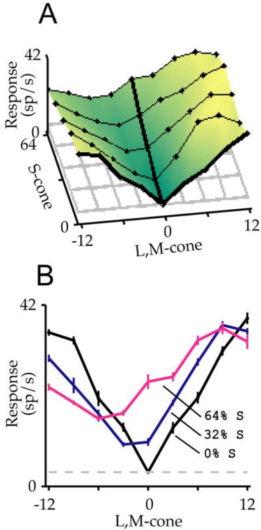
Figure 2. Neural response profile for one neuron. A. 3D surface plot of the neural response to the grid of stimuli. Bold lines highlight the purely L,M- and S-cone contrast response functions. The color scale indicates relative response amplitude, running from zero (dark green) to the maximum firing rate (bright yellow). B. 2D slices through the neural response profile at three S-cone contrast levels. Error bars are standard error of the mean.
