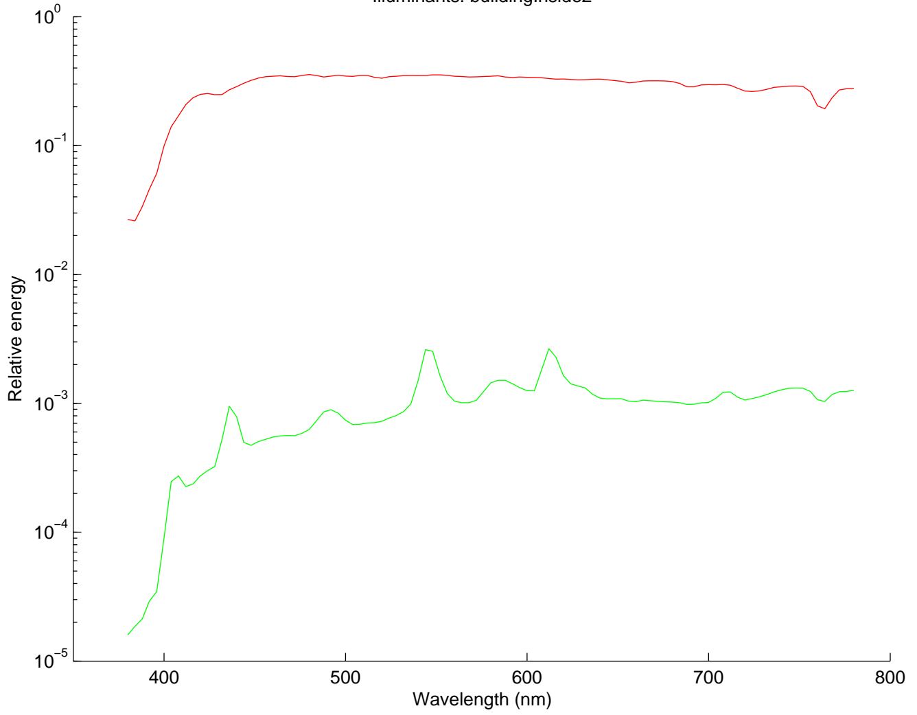
Illuminants: buildingInside2
